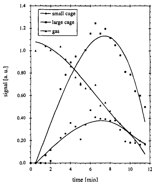
Figure 3. Formation of a xenon clathrate hydrate at 217 K monitored by the change in the integrated intensities of the ^{129}\text{Xe} NMR signals with time t after admission of the xenon. The curves serve merely to guide the eye.
